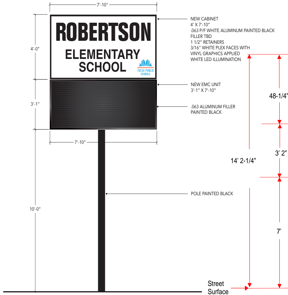
A | ELEVATION SCALE: 3/8" = 1'-0" D/F ILLUMINATED
